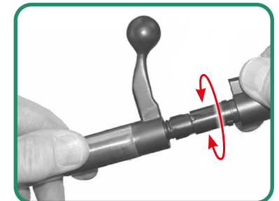
Fig. 9: TITAN 6®: Disassembly of the bolt
